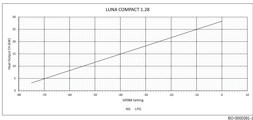
Obr. 58 Graf pro LUNA COMPACT – 1.28
