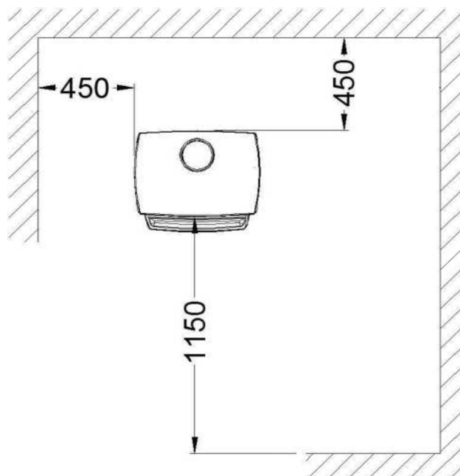
FIG. 6 - SAFETY DISTANCES
